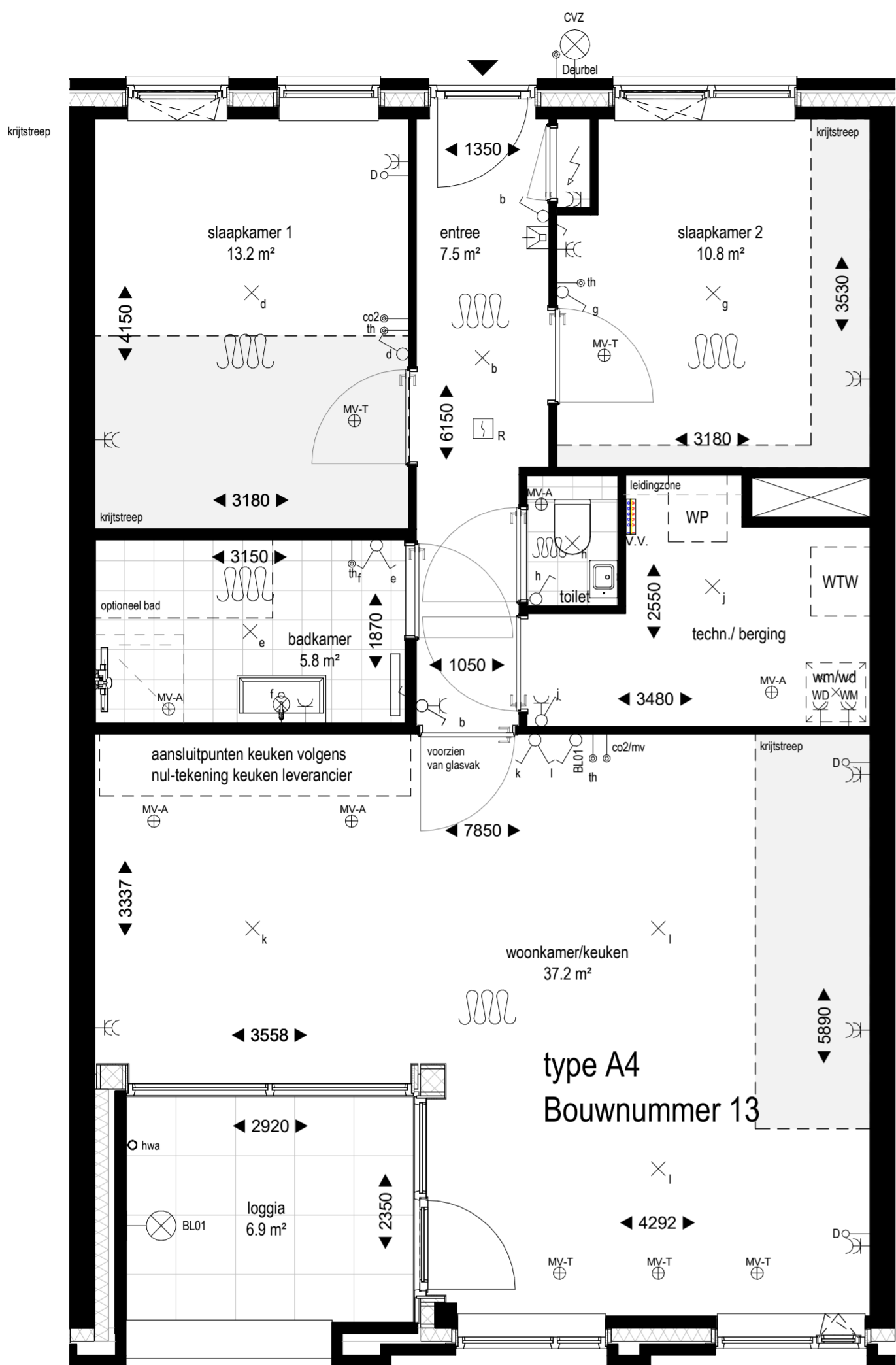
Appartement type A4, bouwnummer 13, 14, 15, 16, 17, 33, 34, 35, 36, 37, 55, 56, 57, 58, 59, 74, 75, 76 en 77
