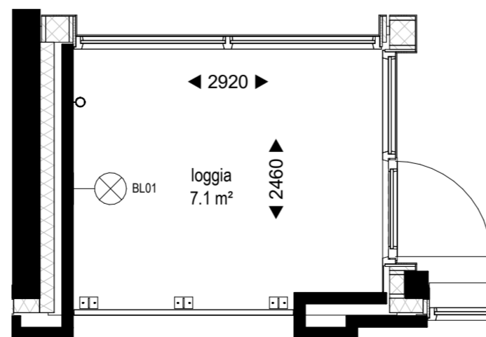
Appartement type A4, loggia bouwnummer 33, 34, 35, 36, 37, 55, 56, 57, 58, 59, 74, 75, 76 en 77
